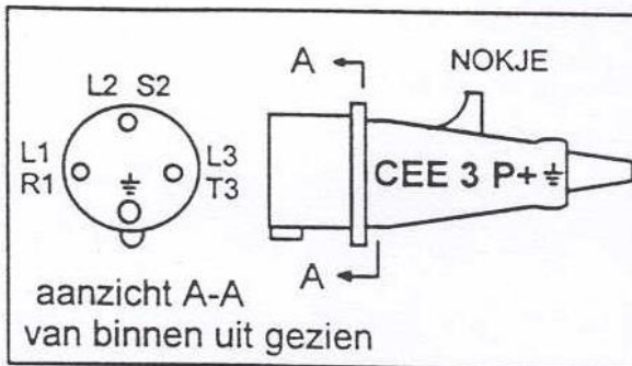
CEE Plug 4pole (3P.+ E⏚)32 A.6h.
